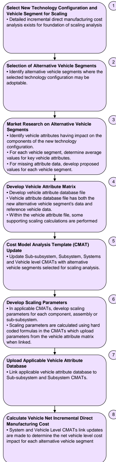
Figure B-7: Process Step Overview for Scaling Incremental Direct Manufacturing Costs to Alternative Vehicle Segments
