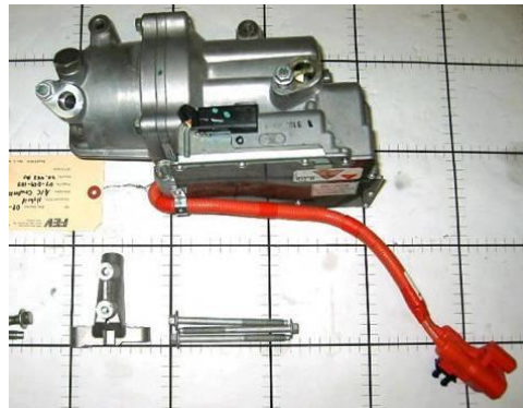
Figure E-6: Electric Compressor and Mounting Hardware
