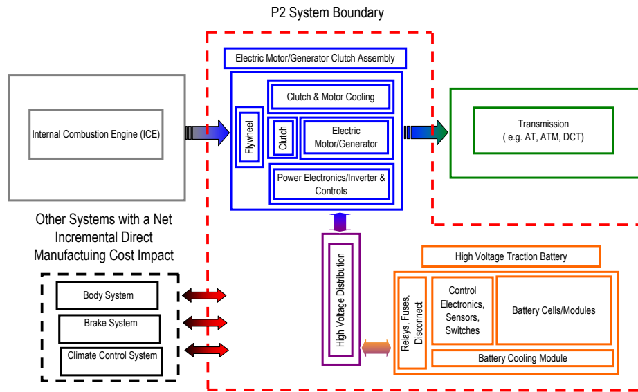
Figure E-4: P2 System Boundary Illustration
