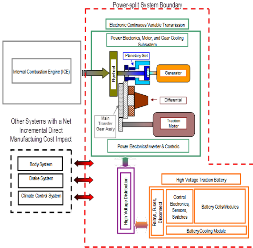
Figure E-3: Power-Split System Boundary Illustration
